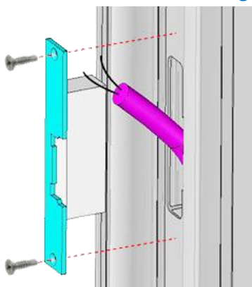
2-Leaf gate
